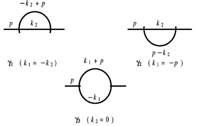
FIG. 2. Subgraphs \gamma_1, \gamma_2 , and \gamma_3 .
